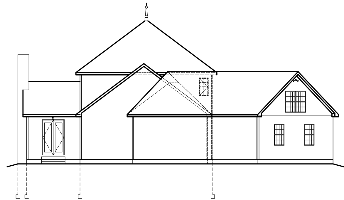
LEFT ELEVATION
