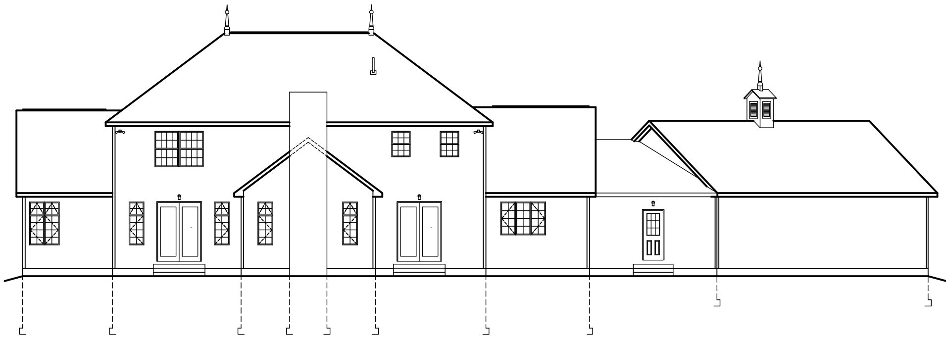
REAR ELEVATION
