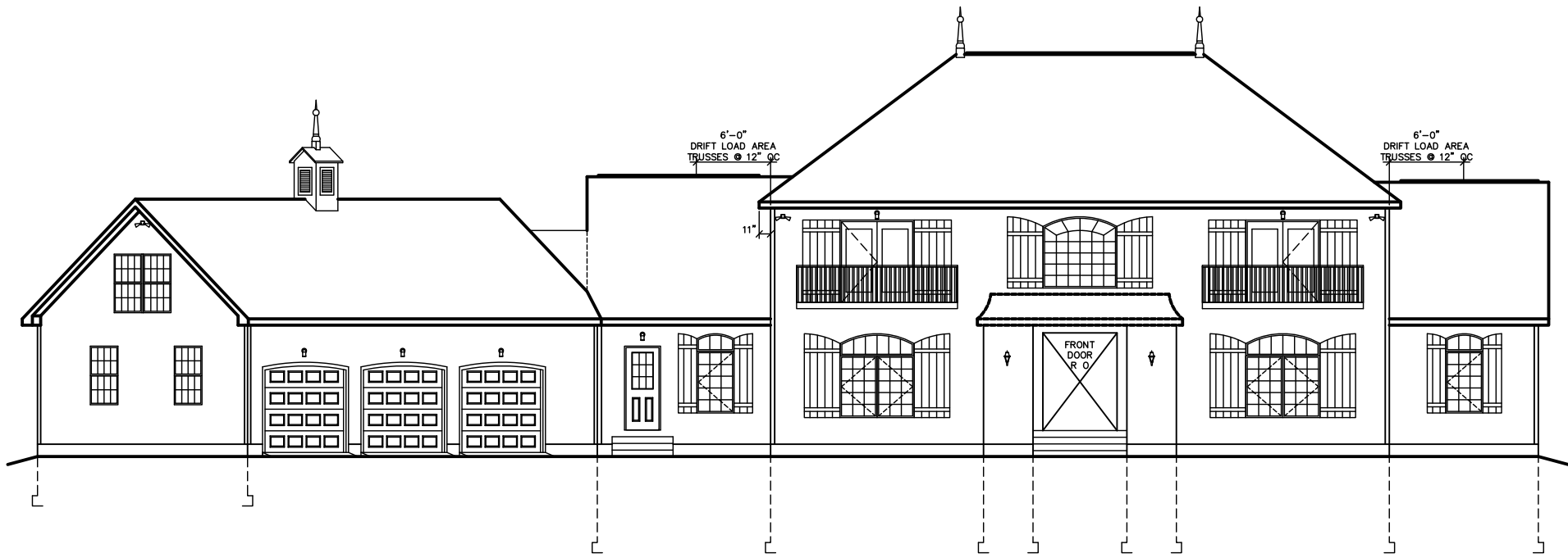
FRONT ELEVATION
