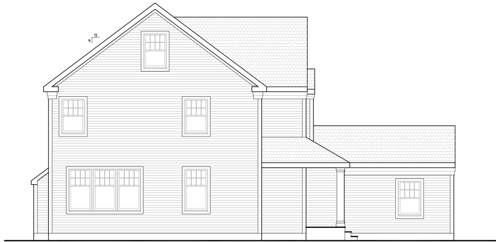
LEFT ELEVATION
